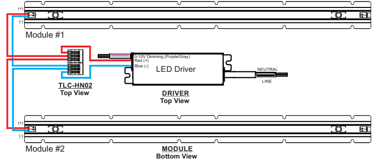
Two Module Wiring (2P)
